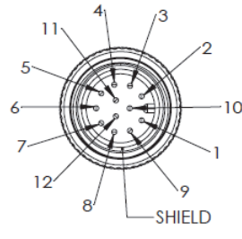
MALE END VIEW (J2)
